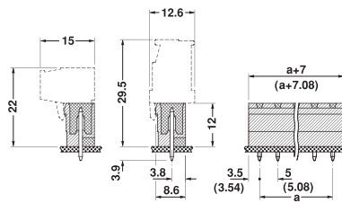
Pitch:5.08(5.00) mm
