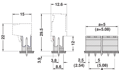
Pitch:5.08(5.00) mm
