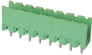
Pitch:5.08(5.00) mm
