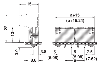
Pitch:5.08(5.00) mm
